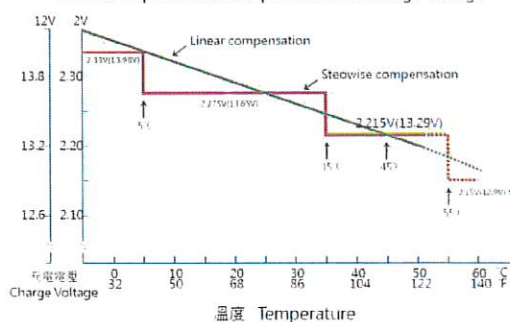
溫度與充電電壓關係 Relationship Between Temperature and Charge Voltage
